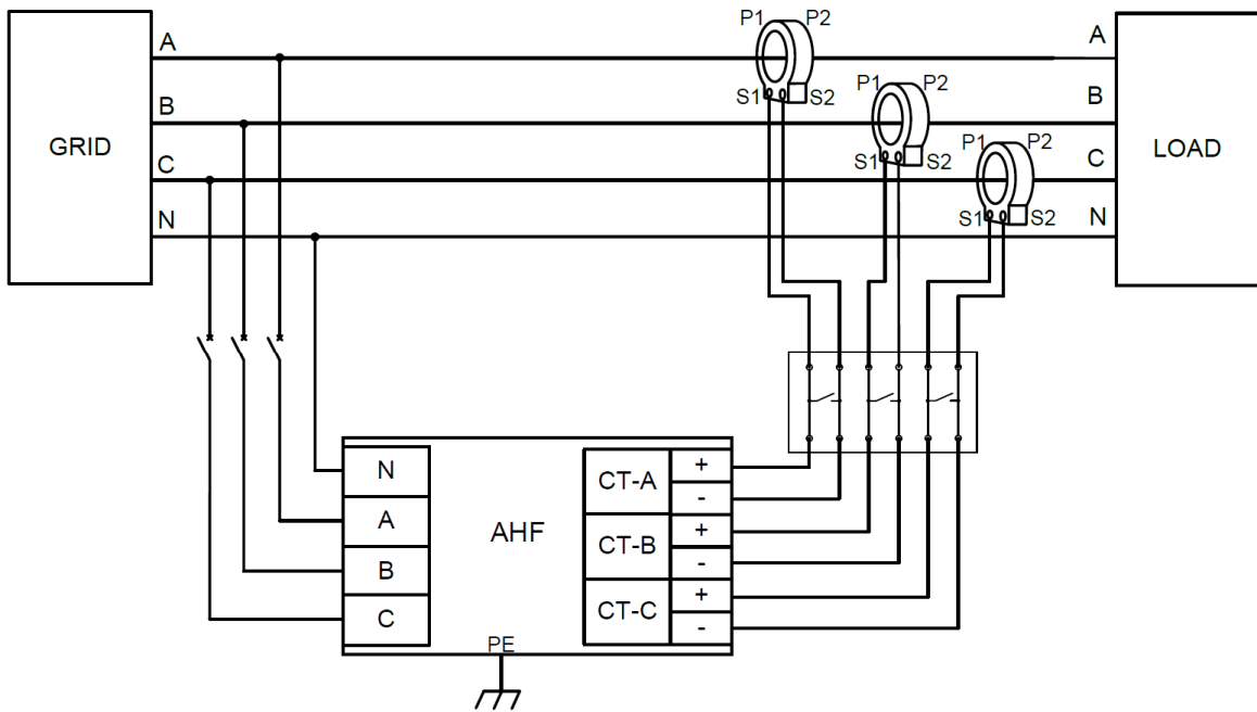
Wiring single power module
